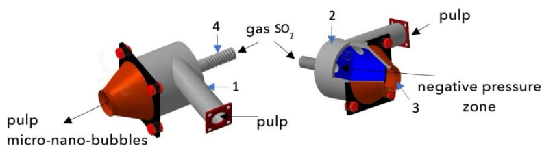
Fig. 2. Hydroacoustic radiator: 1 - pulp supply connection; 2 - resonator chamber; 3 - output connection; 4 - suction connection \text{SO}_2 .
