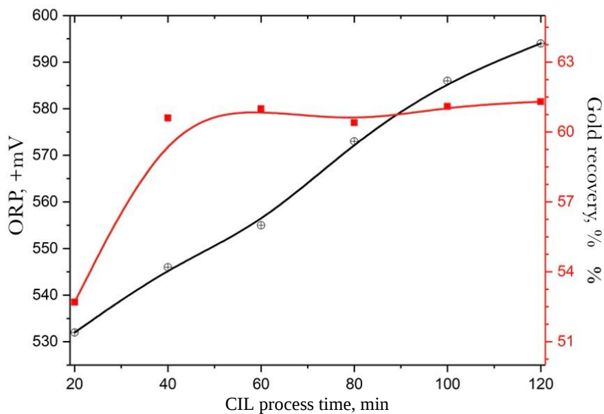
Fig. 3. Slurry potential and gold recovery as a function of the time of the direct CIL process with SO 2 feeding: L:S - 1:3; initial concentration of H 2 SO 4 - 0.5%; iron (III) sulphate loading - 7 kg/t; thiourea loading - 2 kg/t; coal loading - 10 kg/t; slurry supply pressure to the hydroacoustic transmitter inlet - 3 bar, sulphur dioxide supply - 20 kg/t (0.17 kg/t *min), time - 2 hours.
