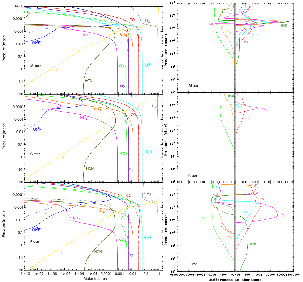
Figure 3. Left: Comparison of the atmospheric composition of GJ 436b using \sigma_{\text{CO}_2}(300 \text{ K}) (dotted line) and \sigma_{\text{CO}_2}(550 \text{ K}) (full line) when the planet orbits an M star (top), a G star (middle) and an F star (bottom). Right: Differences in abundances (in %) between the results obtained with \sigma_{\text{CO}_2}(300 \text{ K}) and \sigma_{\text{CO}_2}(550 \text{ K}) for species that have an abundance superior to 10^{-10} , for an M star (top), a G star (middle), and an F star (bottom).
