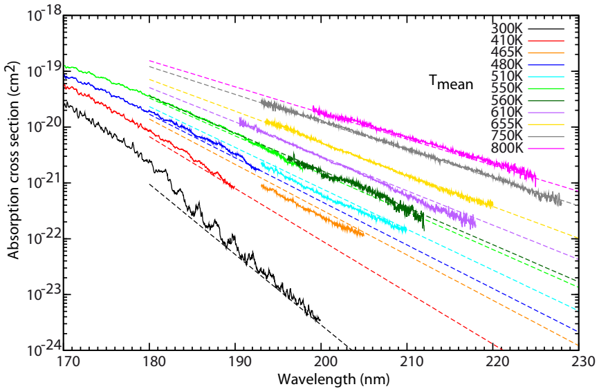
Figure 2. Absorption cross section of \text{CO}_2 for wavelengths longer than 195 nm at 465 K, 510 K, 560 K, 610 K, 655 K, 750 K, and 800 K, plotted with the cross section at ambient temperature (black) and the absorption cross sections measured at shorter wavelengths and presented in Fig. 1 (300 K, 410 K, 480 K, and 550 K). The absorption cross sections calculated with Eq. 1 are plotted with the same color coding.
