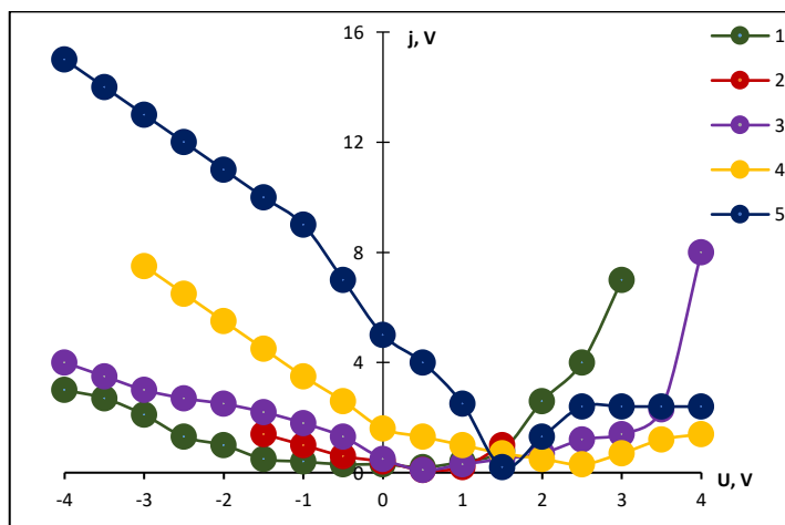
Fig. 3. Dependence of the magnitude of the potential on the bias voltage: 1 \pm x = 1.9 ; 2 \pm x = 1.8 ; 3 \pm x = 1.73 ; 4 \pm x = 1.4 ; 5 \pm x = 1.65 .
