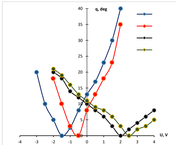
Fig. 4. Dependences of the inclination angle of molecules at the boundary with the germanium type substrate 1 ( T = 20^\circ\text{K} ), 2 ( T = 40^\circ\text{K} ); n-type- 3 ( T = 20^\circ\text{K} ), 4 ( T = 40^\circ\text{K} ) on the bias voltage.
