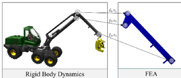
Fig. 3. Interface between RBD Simulation and FEA Simulation.
