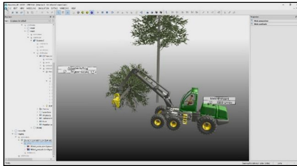
Fig. 1. Real-life application scenario for the developed concept and implementation: A harvester is cutting a tree. The DT of the mobile machinery builds the base for enhanced structural mechanics.
